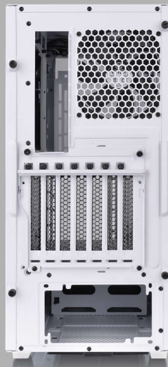
Vertical VGA Bracket installation
